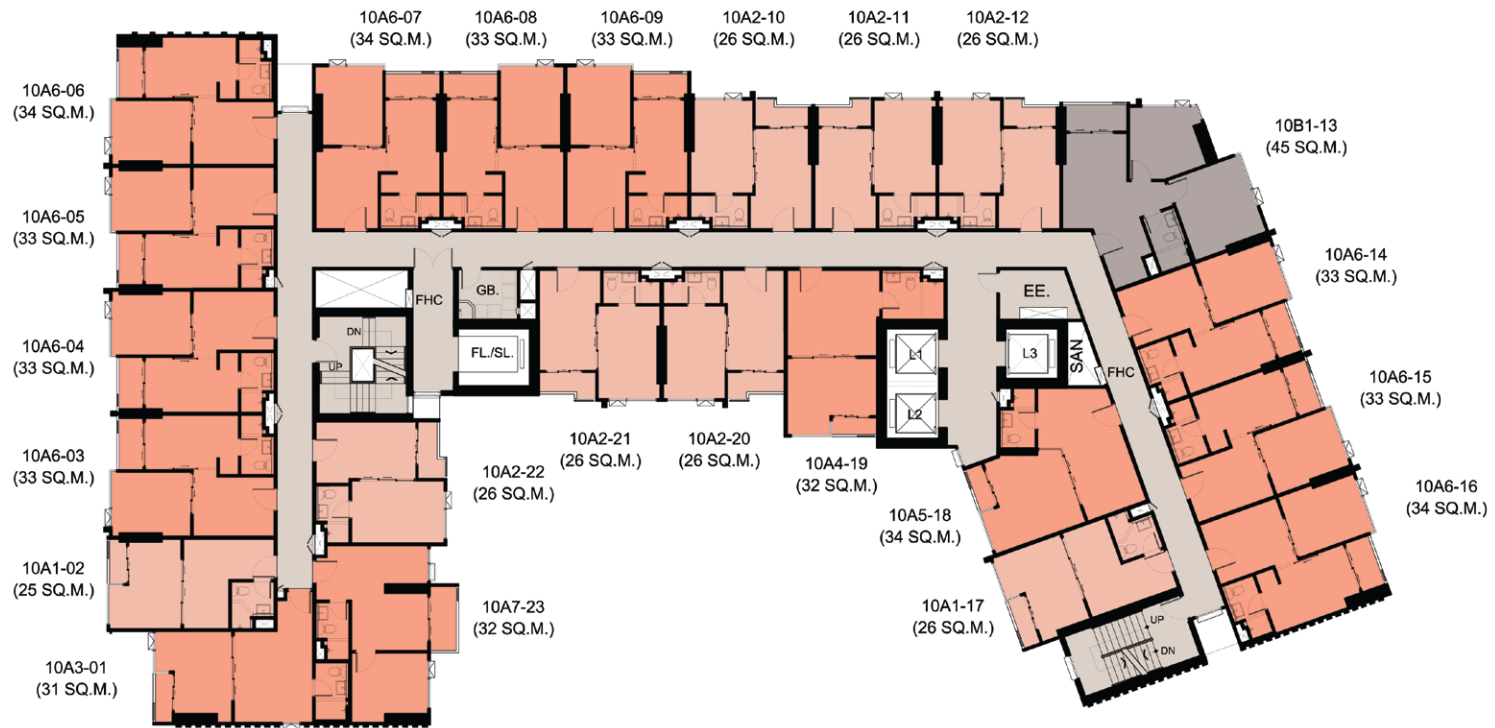
10th , 11th , 12Ath , 14th , 16th , 17th , 19th , 20th , 22nd FLOOR PLAN
